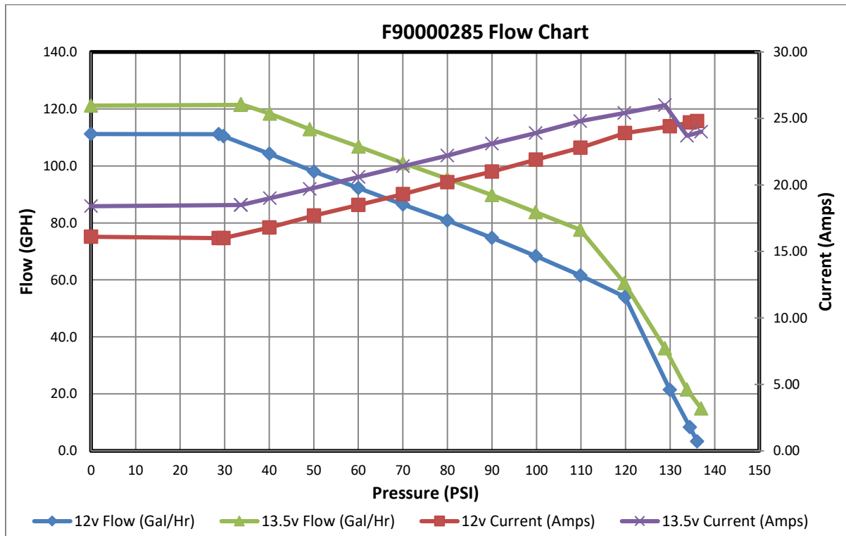
F90000285: Flex Fuel HP Pump
